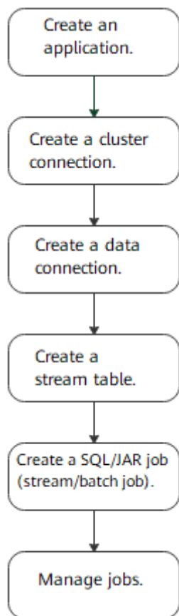
Figure 6-11 Flink web UI application process
