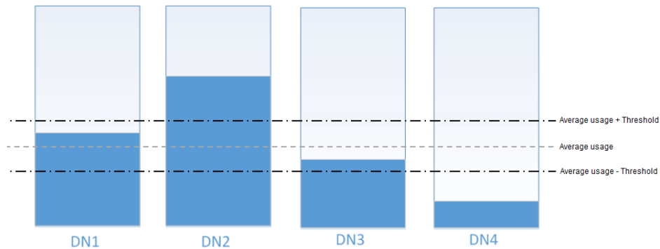
Figure 9-6 DataNode disk usage before balancing
