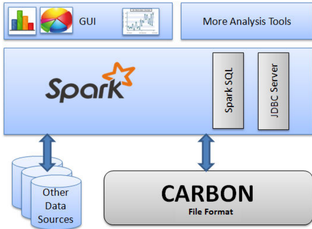
Figure 3-1 Basic architecture of CarbonData
