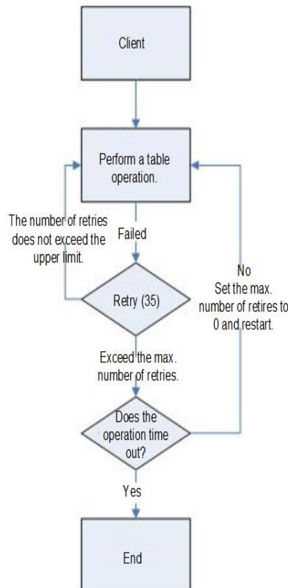
Figure 8-3 Process for HBase client operation retry timeout
