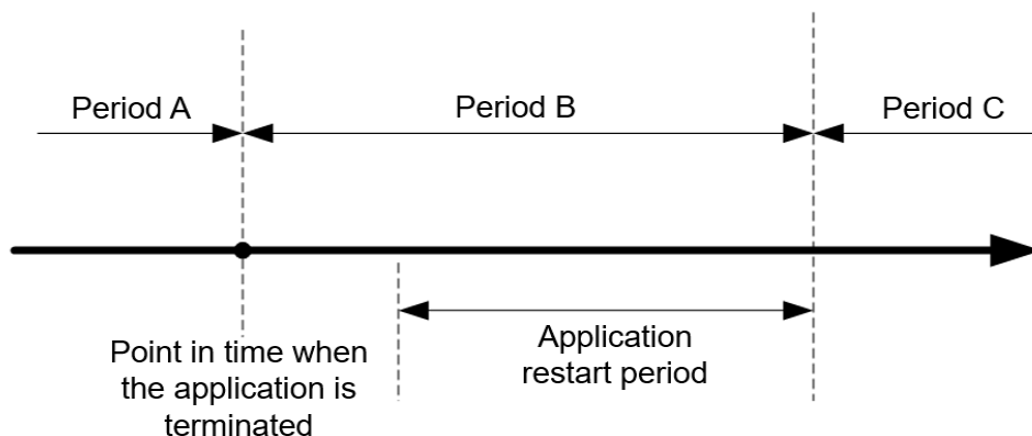
Figure 26-5 Time axis for restarting the Spark Streaming application
