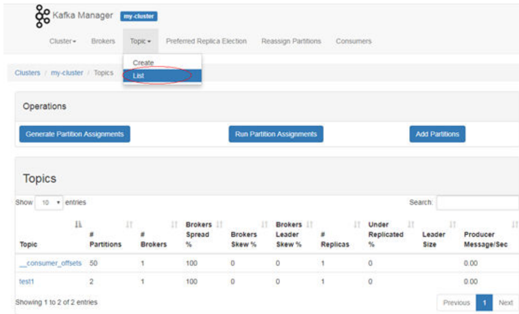
Figure 16-7 Topic list
