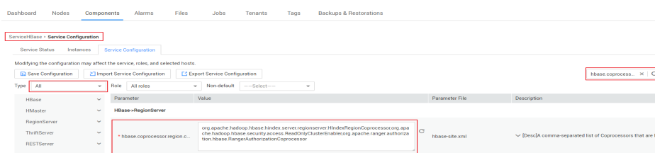
Figure 23-15 hbase.coprocessor.region.classes
