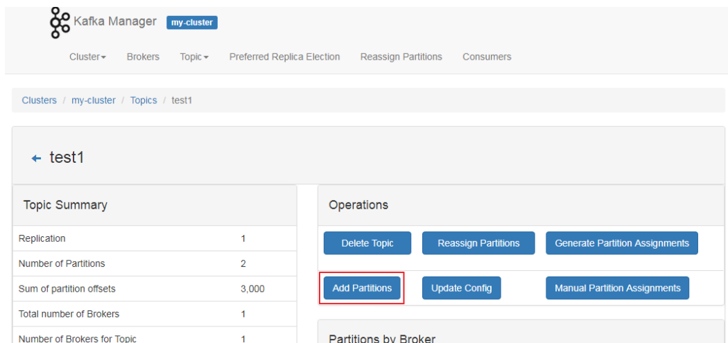
Figure 16-12 Adding partitions
