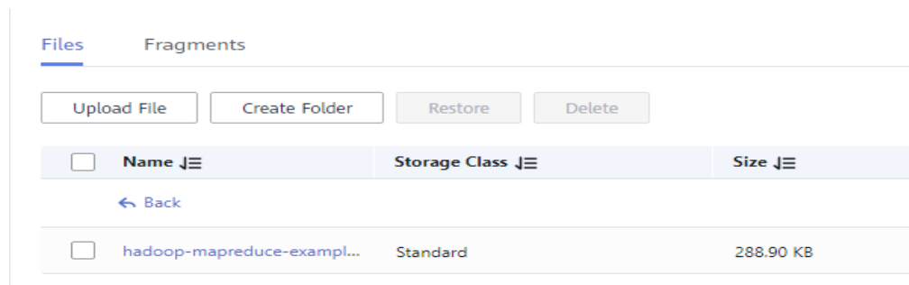
Figure 9-2 Program list
