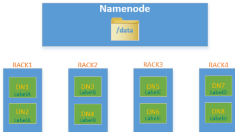
Figure 9-12 Scenario example
