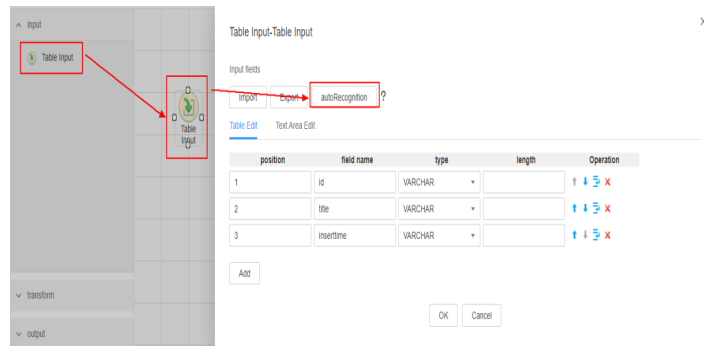
Figure 17-38 Operator input
