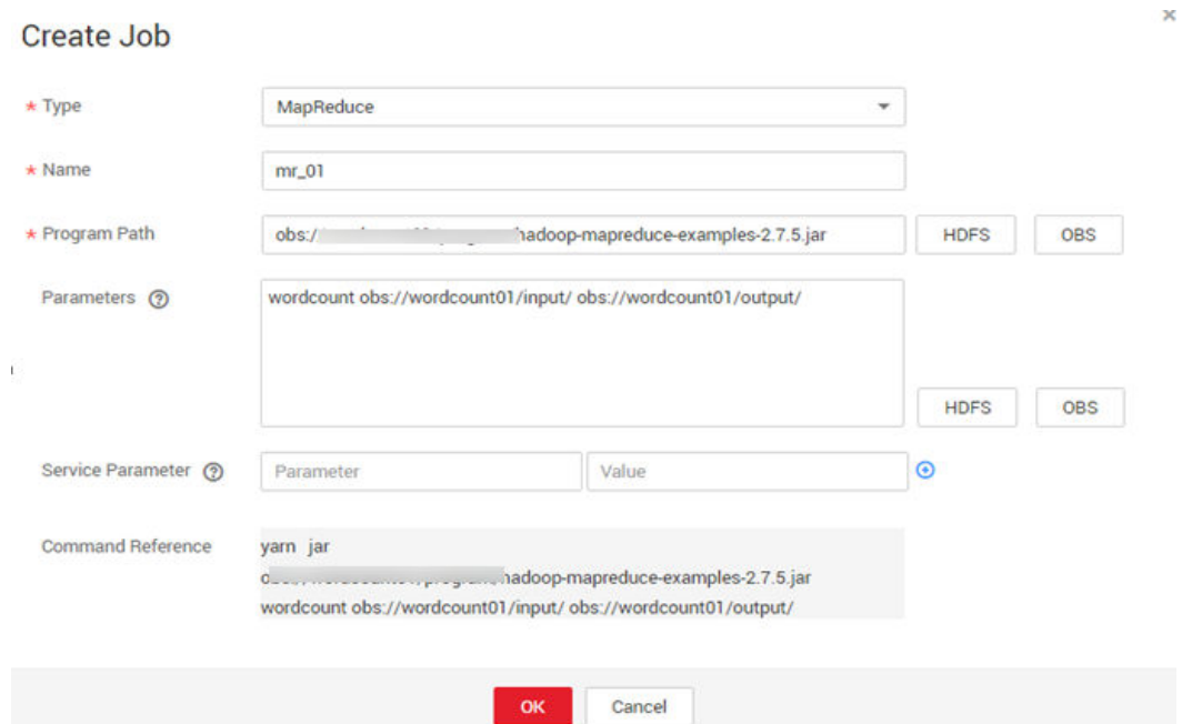
Figure 9-4 wordcount job
