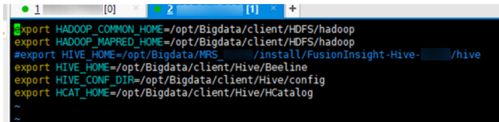
Figure 27-3 Setting environment variables of Sqoop
