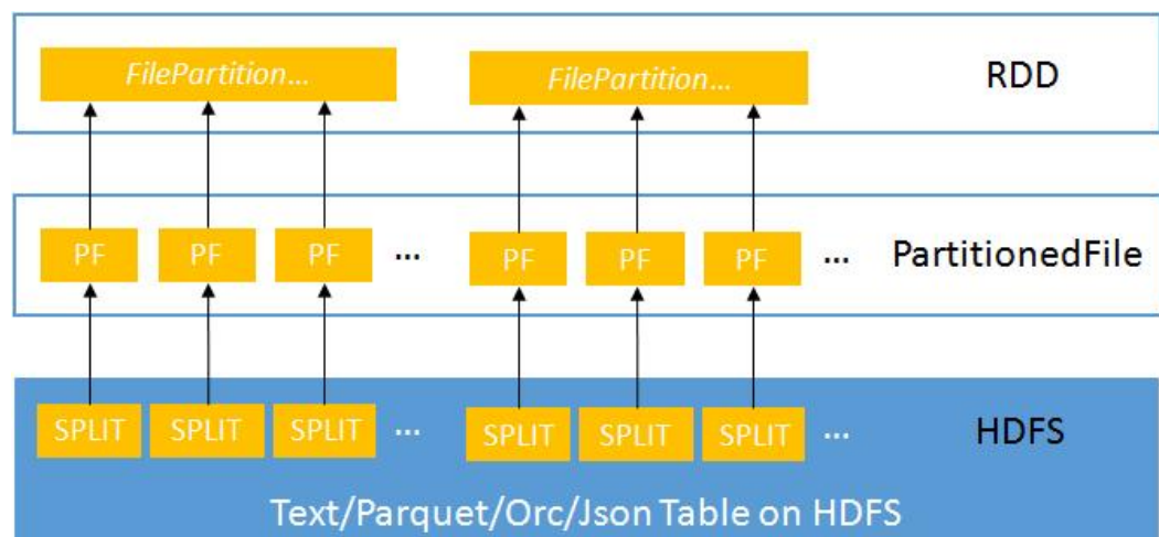
Figure 26-8 Merging small files
