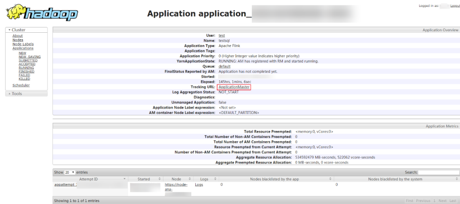
Figure 6-9 Application
