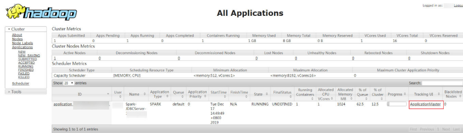
Figure 25-5 ApplicationMaster
