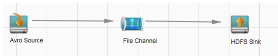
Figure 7-19 Example for the Flume configuration tool
