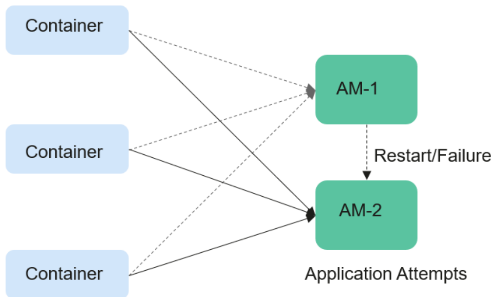
Figure 30-1 ApplicationMaster job preserving
