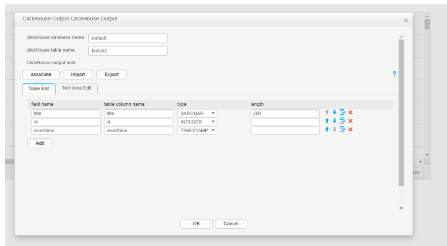
Figure 17-39 Operator output
