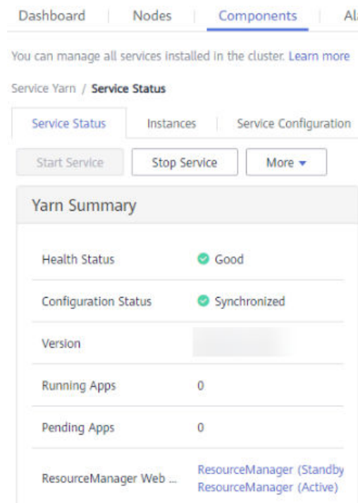
Figure 6-10 Yarn summary
